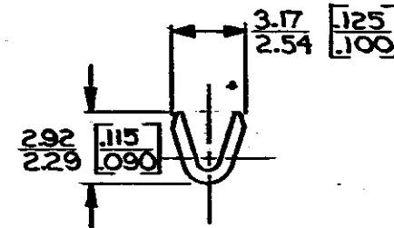
SECT. A-A
